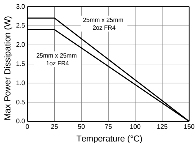
Figure 2. Derating Curve
