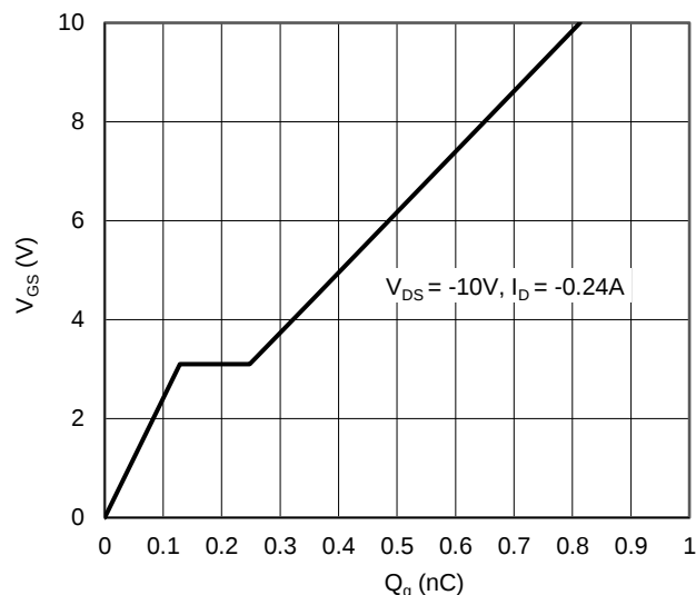
Figure 22. Gate Charge (Q2)
