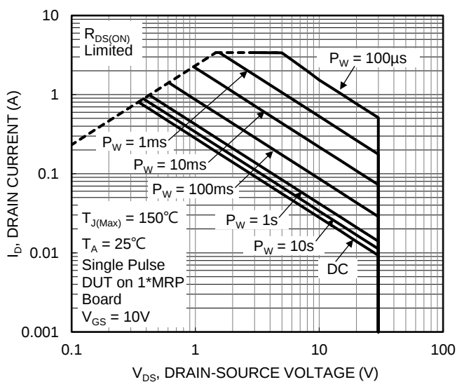
Figure 23. SOA, Safe Operation Area (Q1)
