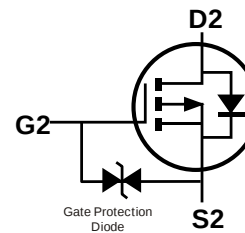
Q2 P-CHANNEL
