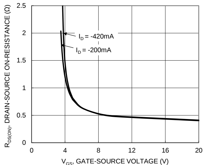
Figure 8. Typical Transfer Characteristic (Q2)
