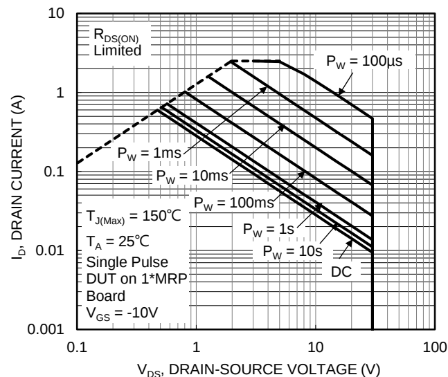
Figure 24. SOA, Safe Operation Area (Q2)
