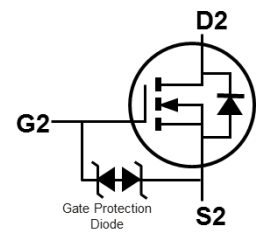
Q2 N-Channel
