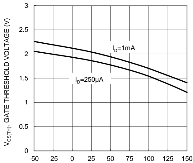
T_J , JUNCTION TEMPERATURE (°C) Figure 7. Gate Threshold Variation vs. Junction Temperature
