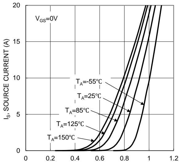
V_{SD} , SOURCE-DRAIN VOLTAGE (V) Figure 8. Diode Forward Voltage vs. Current
