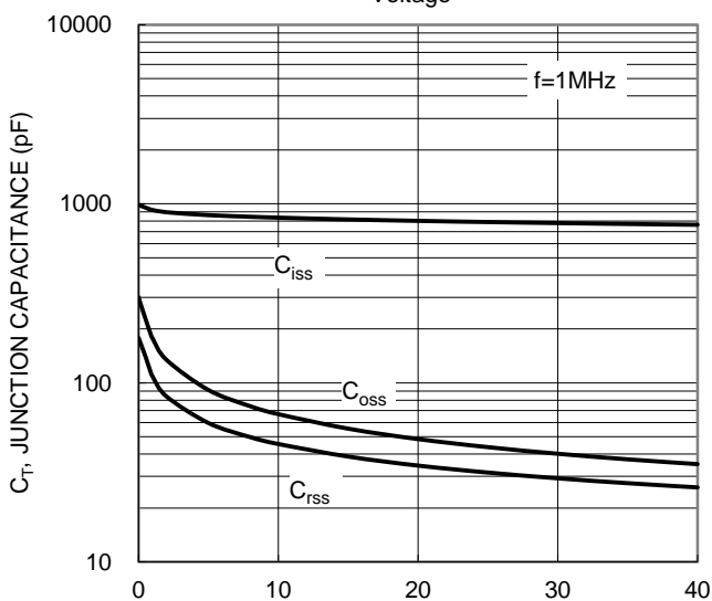
V_{DS} , DRAIN-SOURCE VOLTAGE (V) Figure 11. Typical Junction Capacitance
