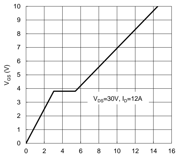
Figure 10. Gate Charge
