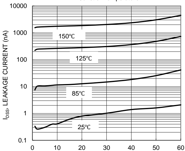
V_{DS} , DRAIN-SOURCE VOLTAGE (V) Figure 9. Typical Drain-Source Leakage Current vs. Voltage
