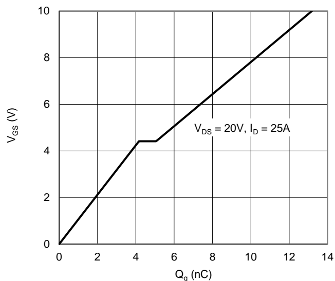
Figure 11. Gate Charge
