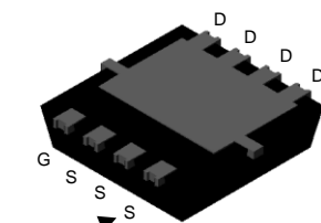
Pin 1 Bottom View
